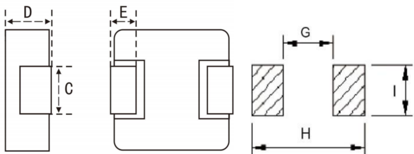
Recommended pad size 推荐焊盘尺寸
